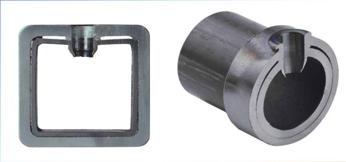
Flowdrilling through 2 materials
